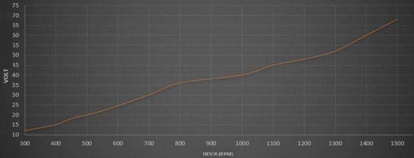
800G-24V-Generator-Rpm-Volt-Graphic
