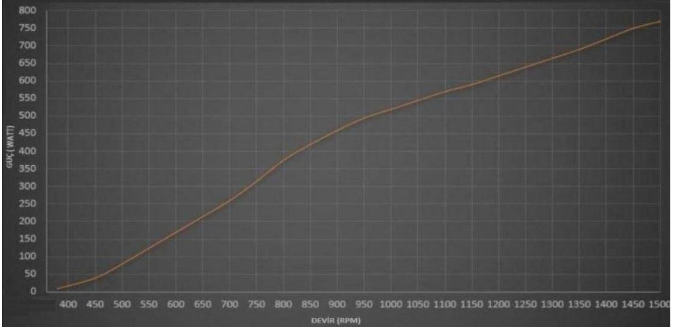
800G-Generator-Rpm-Power-Graphic
