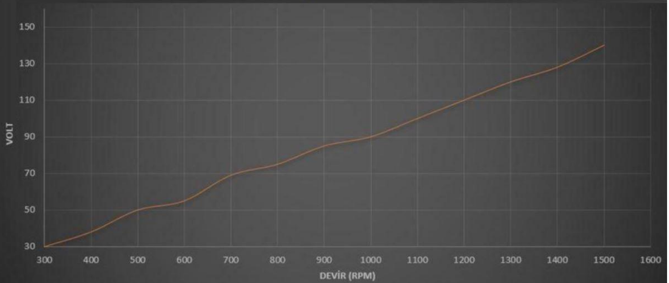
800G-24V-Generator-Rpm-Volt-Graphic
