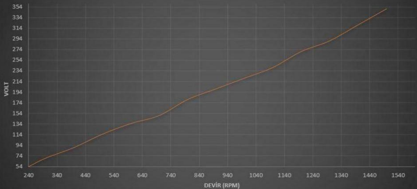
800G-48V-Generator-Rpm-Volt-Graphic
