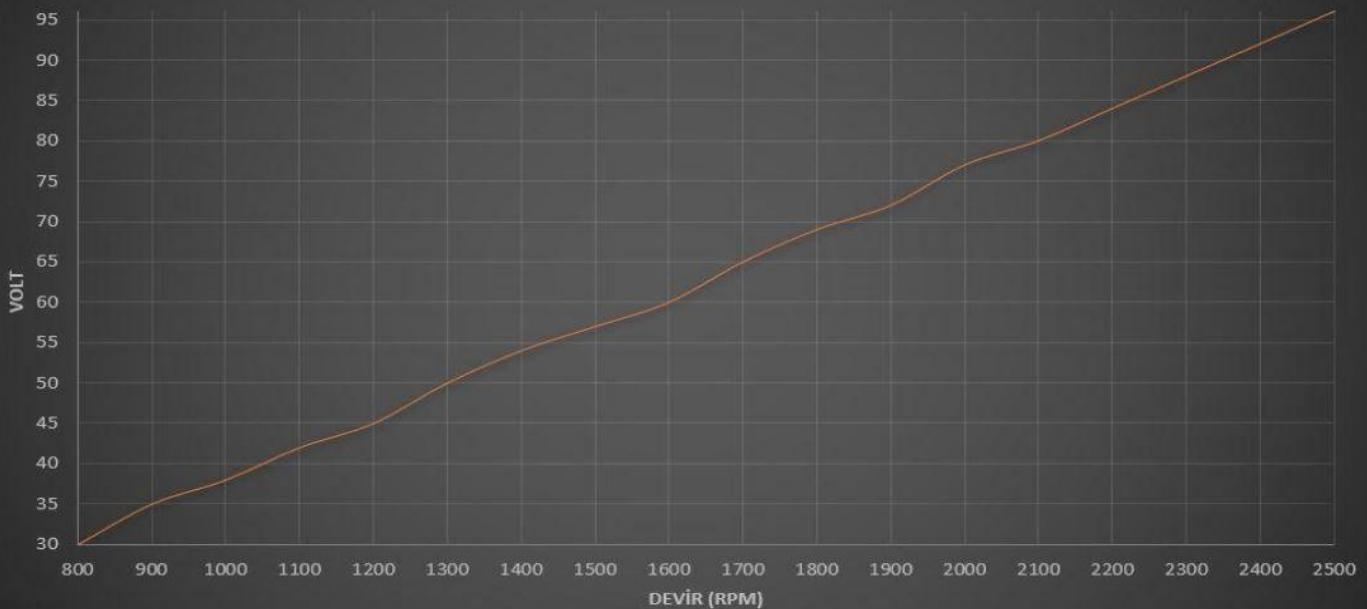
500G-24V-Generator-Rpm-Volt-Graphic
